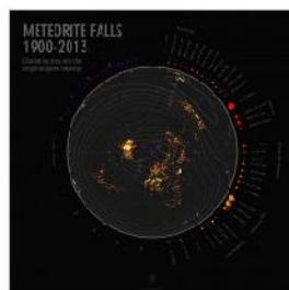
Meteorite Falls 1900-2013
