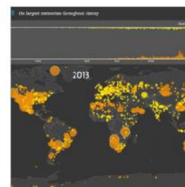
Macrometeorites
