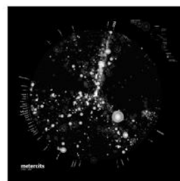
meteorites 1900 - 2000
